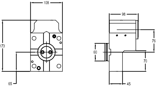
图纸：45 C5-L/RCE-NL3000-076098A
