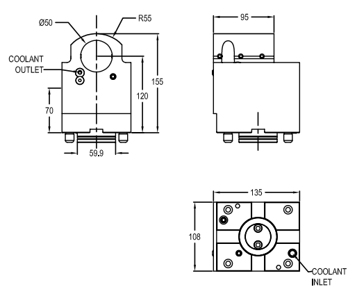
图纸：21 T10114
