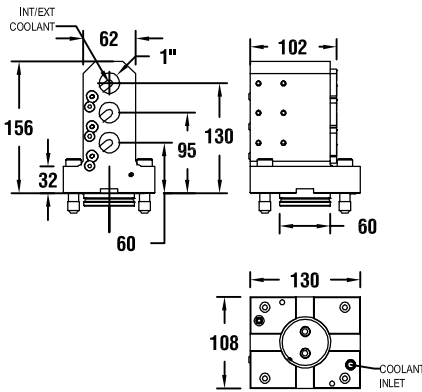
图纸：27 T10108
