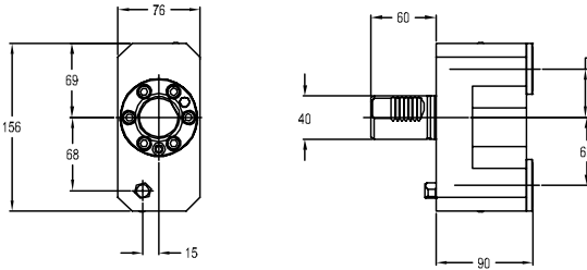
图纸：65 C4-L/RCE-SQT10-000090MDT
