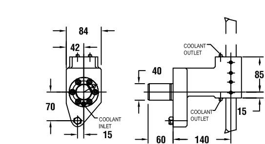
图纸：92 53638000400
