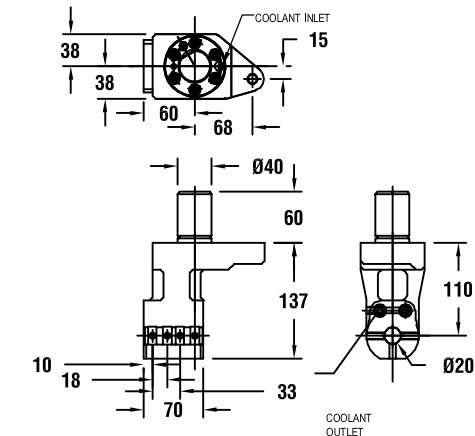
图纸：59 53538000201
