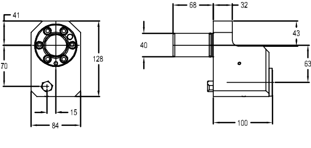
图纸：22 C4-L/RCE-MZ6200-063100M
