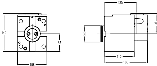
图纸：52 C4-L/RCI-NT4200-120075A
