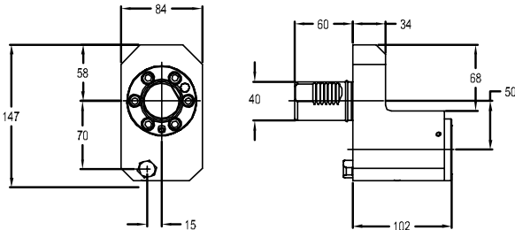
图纸：99 C5-L/RCE-SQT250-050102MSS
