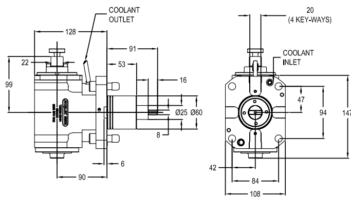
图纸：7 T32226-22MM
