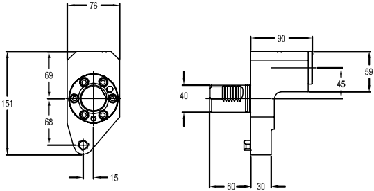
图纸：63 C4-L/RCE-SQT10-045090M
