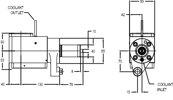
图纸：73 C4-DTI-QTN200-130060I
