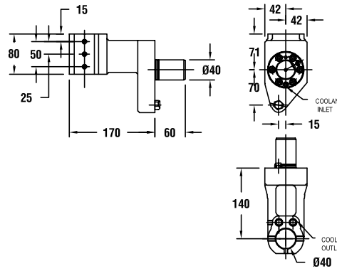
图纸：90 53208005100
