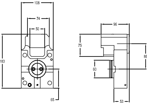
图纸：43 C5-L/RCE-NL3000-086053A
