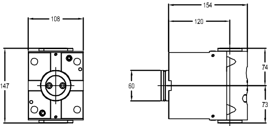
图纸：54 C4-L/RCI-NT4200-120075ADT
