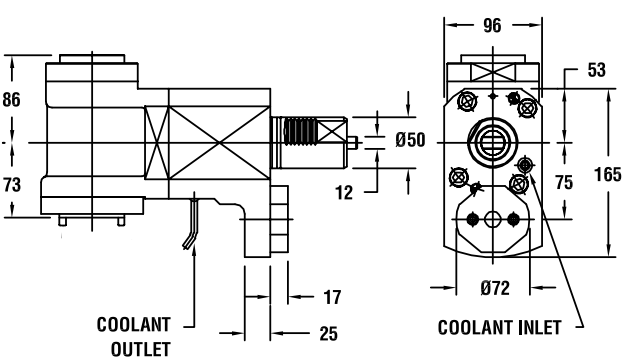
图纸：26 198.15834.000
