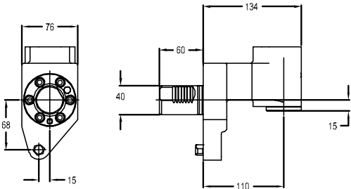
图纸：67 C4-L/RCI-SQT10-110015MSS
