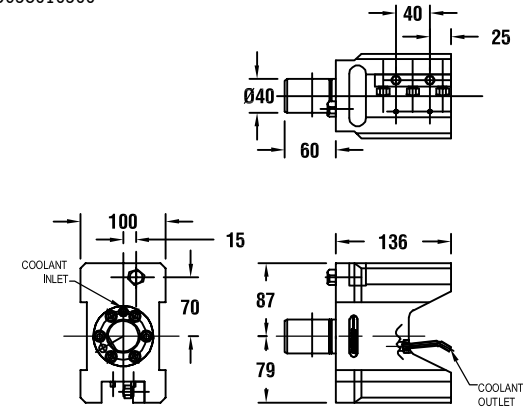
图纸：86 53638010300
