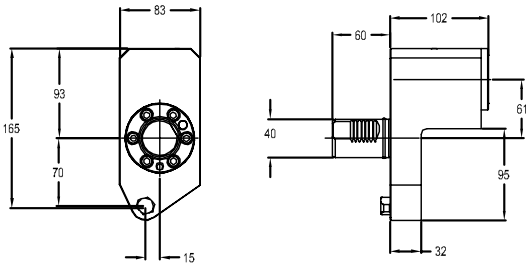
图纸：97 C5-L/RCE-SQT250-061102M
