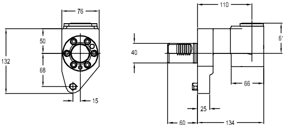
图纸：66 C4-L/RCI-SQT10-110061M
