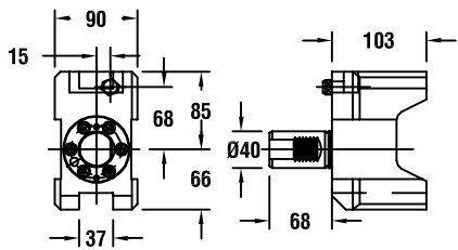
图纸：52 53538000101
