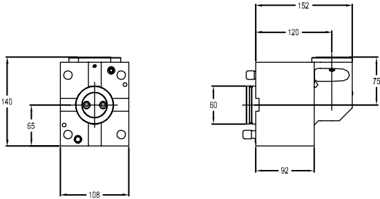
图纸：51 C5-L/RCI-NT4200-120075A
