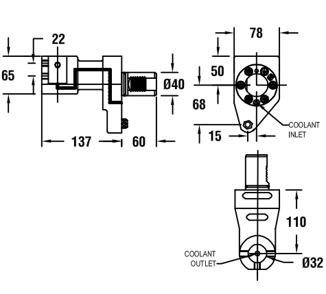
图纸：61 53518000501
