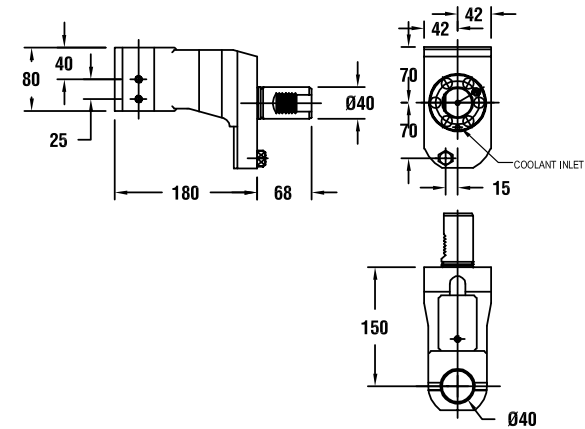
图纸：21 53478000801
