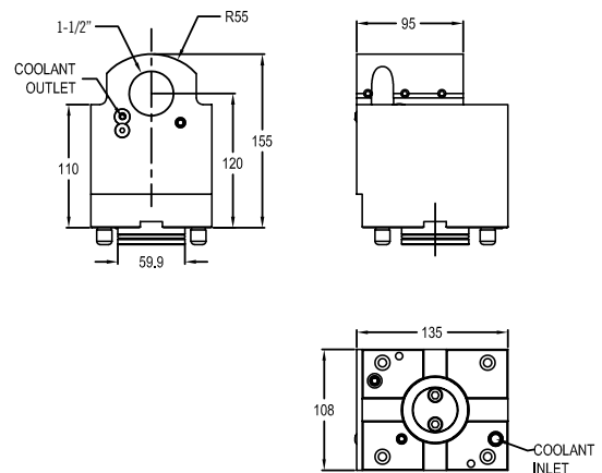
图纸：22 T10134
