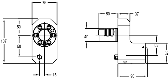
图纸：64 C4-L/RCE-SQT10-063090MSS
