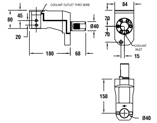
图纸：20 53478002200
